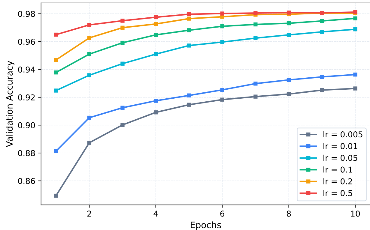
Validation Accuracy across Learning Rates
