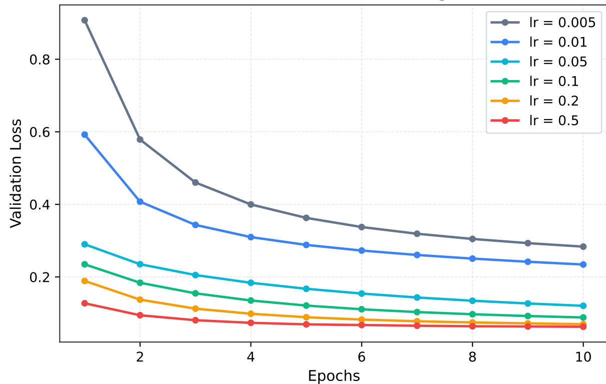
Validation Loss across Learning Rates
